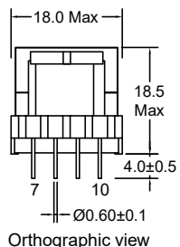
Orthographic view
